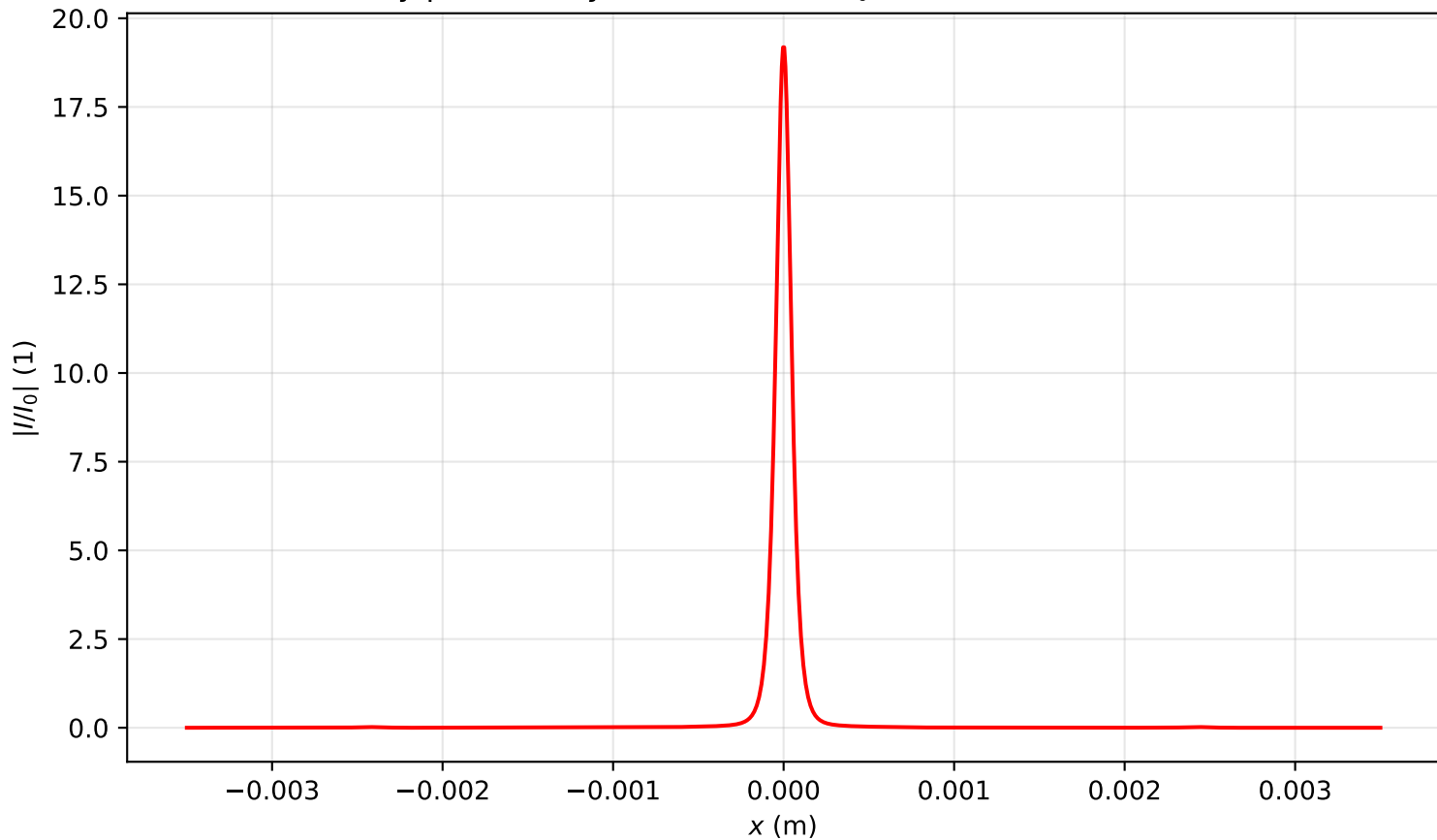
Intensity profile I(x, y = 0, z = 3.821)/I_0 , P_{in}=2.5P_{cr} , artificial time
